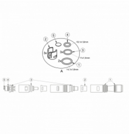
Spare part kit COAX® cartridge MIDI 0109531 Spare part kit Midi COAX(Piab)
